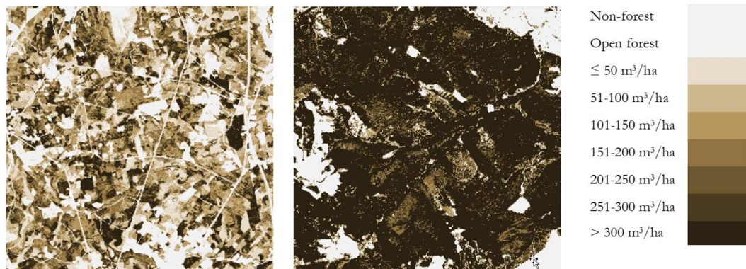
Figure 3: Stem volume maps computed in the first pilot services Forest Flux on 7 km x 7 km areas in Finland and Romania. The relative RMSE was in Finland 52% and bias 0.1 m 3 /ha and in Romania 59% and 2.3 m 3 /ha, respectively. The uncertainties were computed at the level of ground sample plots using an independent plot sample. The uncertainties are smaller for larger areas.
